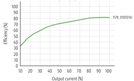
Efficiency vs output load
